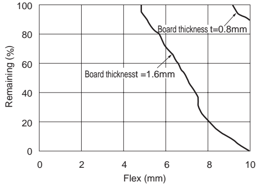
Relation between board thickness and flex strength (C1608X7R1C103K)
